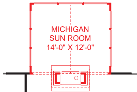
14' X 12" MICHIGAN ROOM AT FAMILY ROOM WITH OPTIONAL SEE-THRU FIREPLACE
