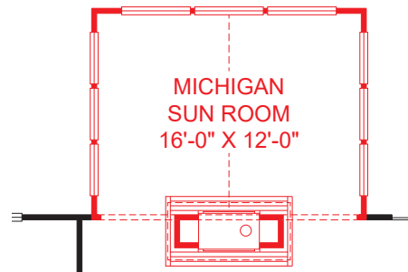
16' X 12" MICHIGAN ROOM AT FAMILY ROOM WITH OPTIONAL SEE-THRU FIREPLACE
