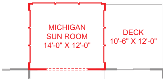
14' X 12" MICHIGAN ROOM
