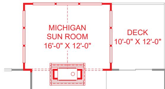
16' X 12" MICHIGAN ROOM WITH OPTIONAL SEE-THRU FIREPLACE
