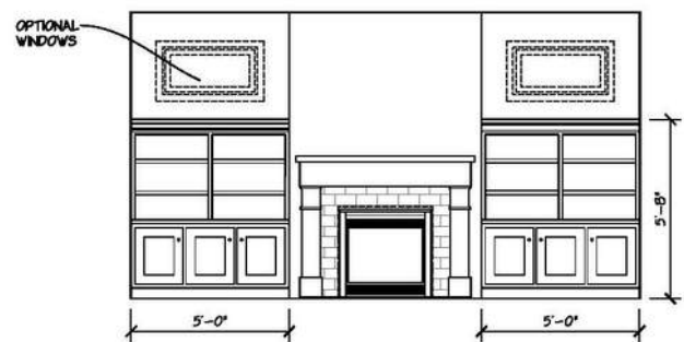
Bookcases with Transom Windows Above 4" Wide Cabinetry | 5" Wide Cabinetry
